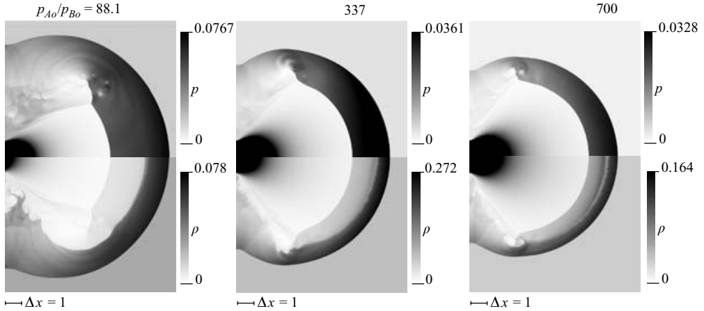
FIGURE 11. Pressure (upper half) and density (lower half) fields in round jets of initial strengths p_{Ao}/p_{Bo} = 88.1 , 337 and 700 taken at times t = 9.54 , 6.19 and 4.98 respectively such that the interface separating driven and driver gases is at the same x location.
